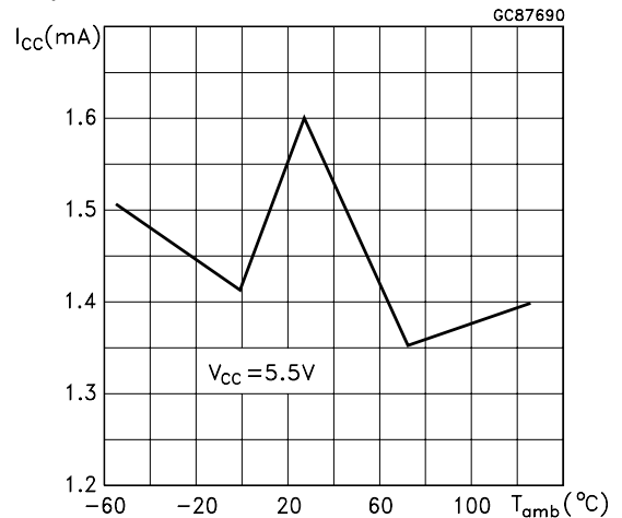
Figure 5 : Driver Short Circuit Supply Current vs Temperature
